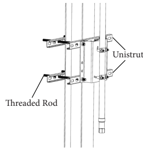
I-Beam (Column) Installation
