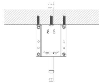
Concrete Roof Installation
