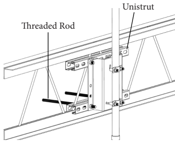
Truss (Purlin) Installation
